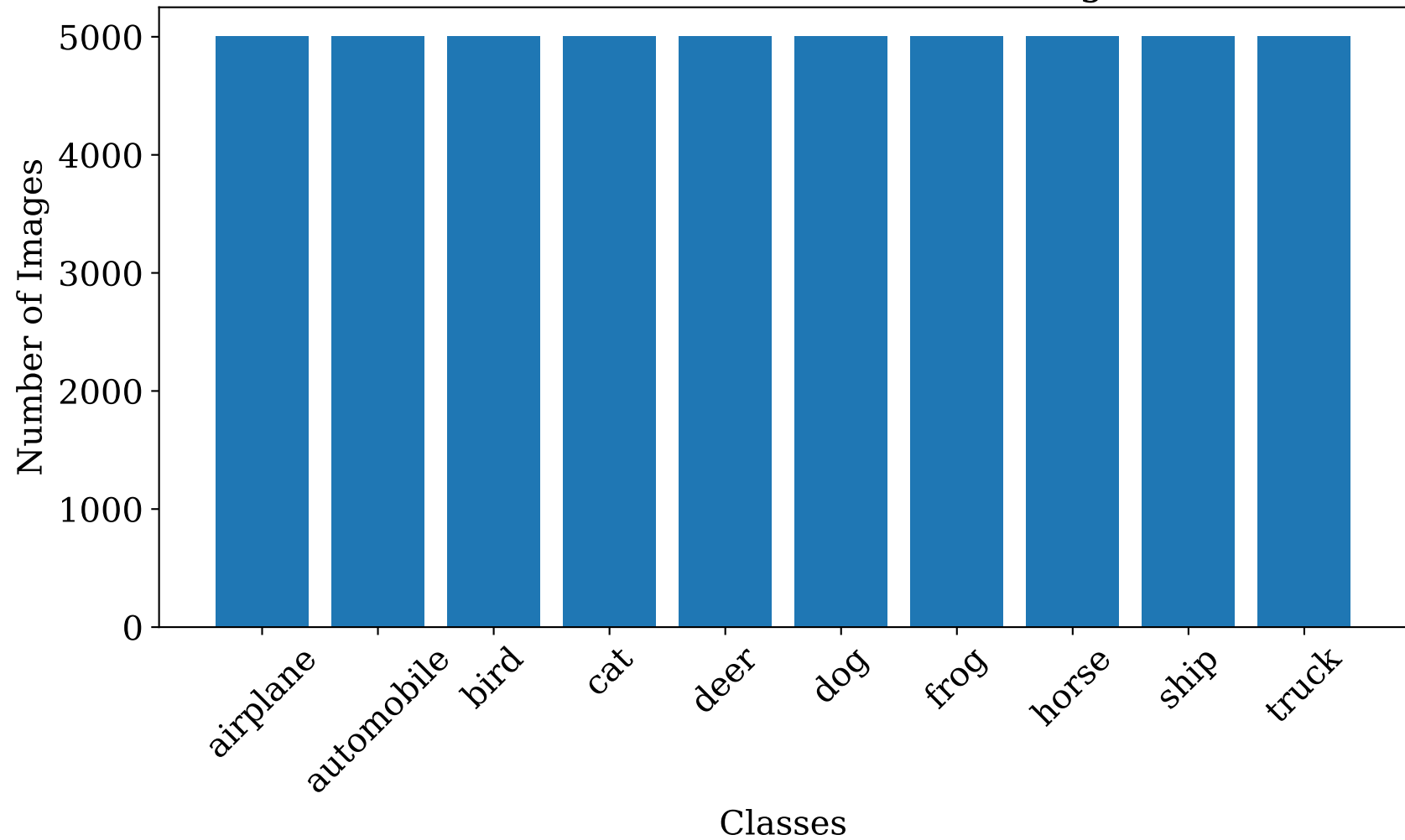
Class Distribution in CIFAR-10 Training Dataset
